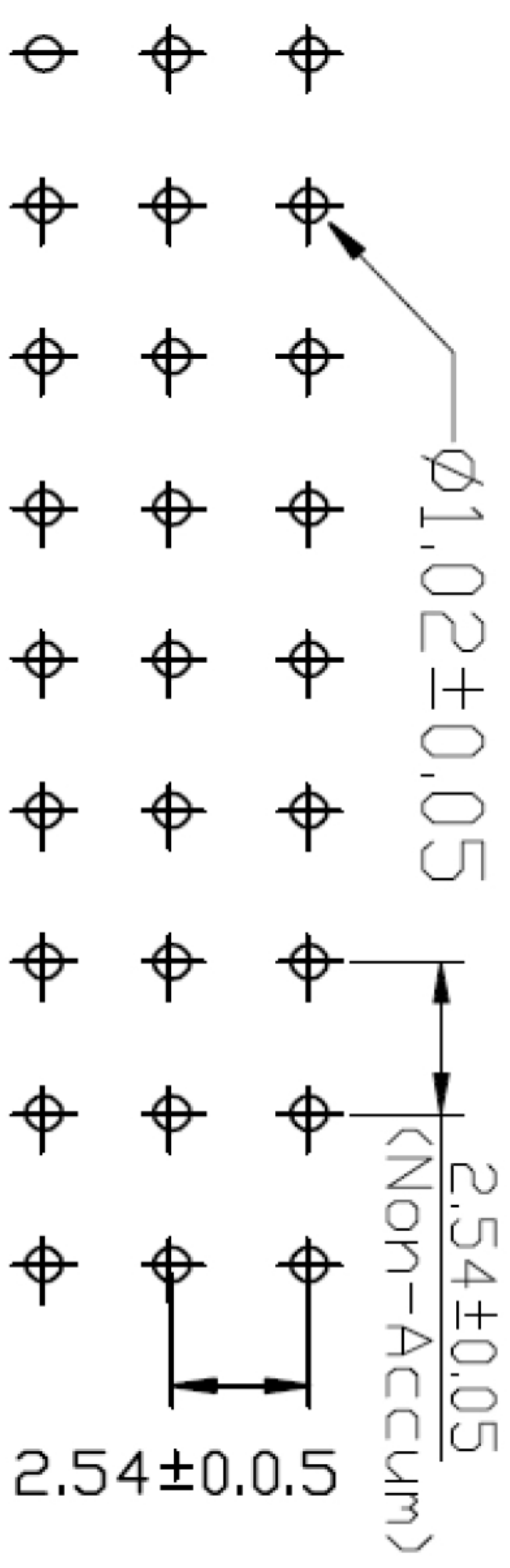
PCB Layout
