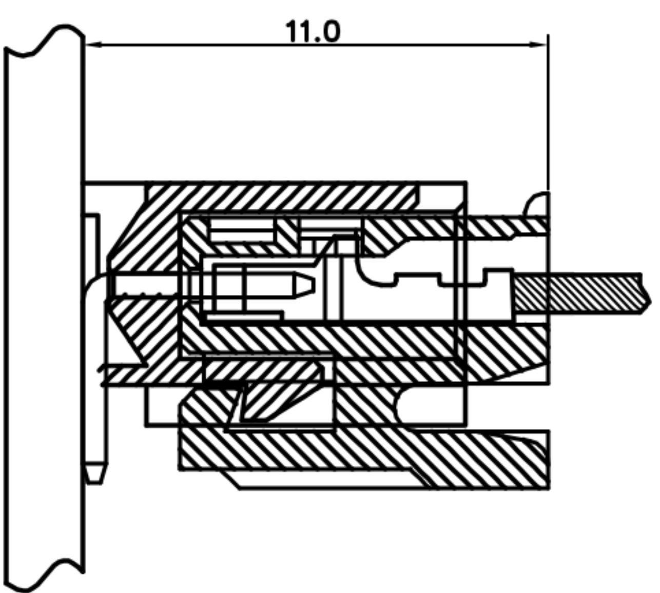
PHB Receptacle + PHB Header
